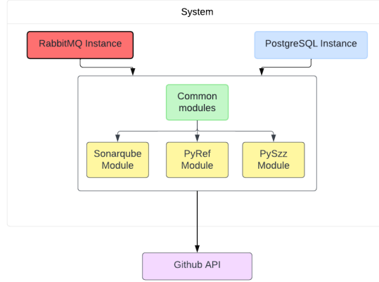
FIGURE 1. PyDs Architecture Diagram
