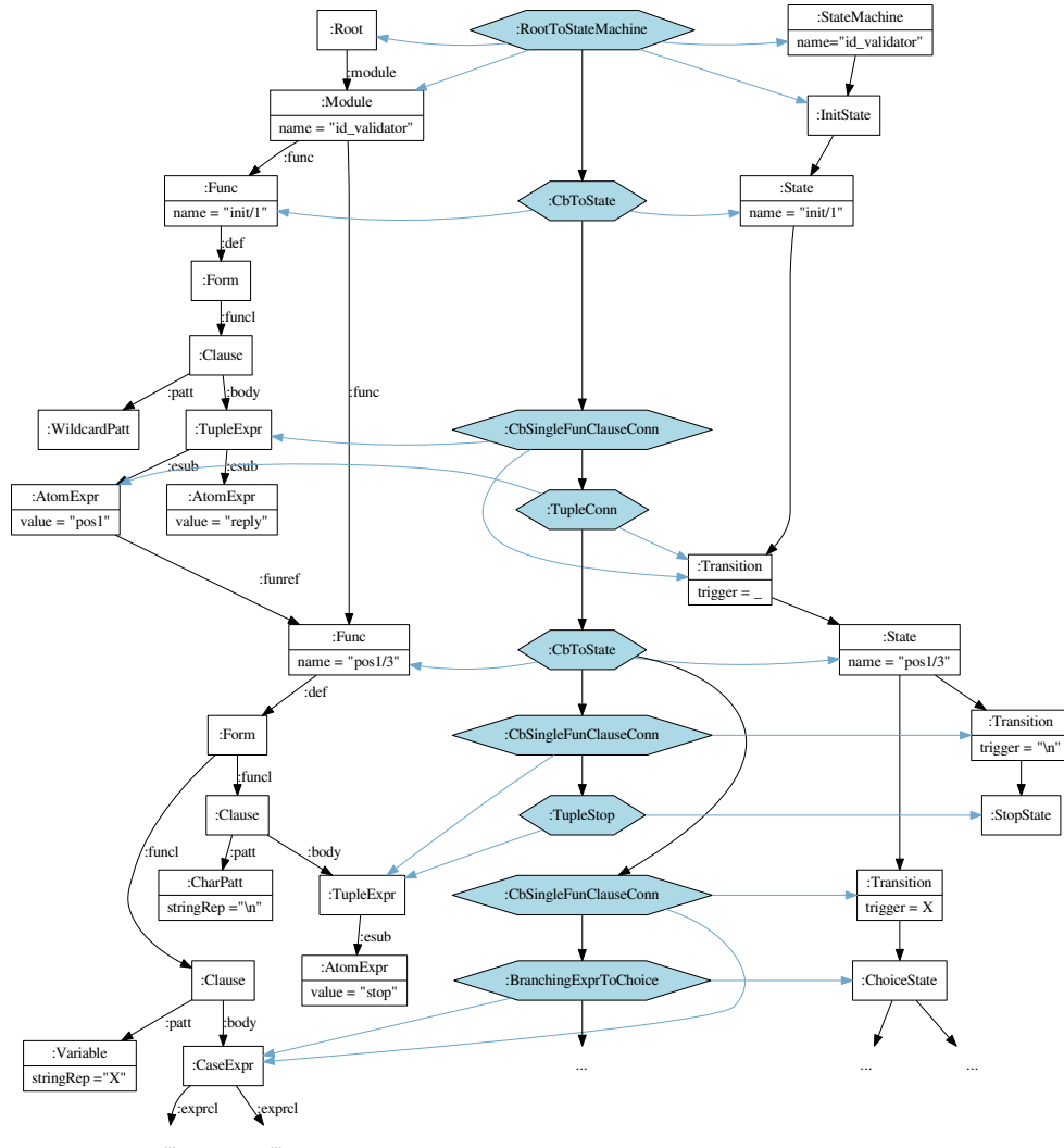
FIGURE 5. Partial trace of the transformation applied to the SPG of the Erlang state machine in Figure 4a
