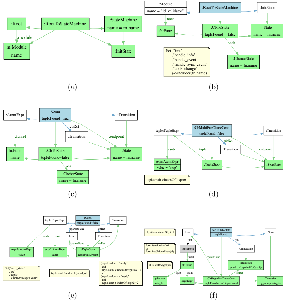
FIGURE 3. Example TGG transformation system
