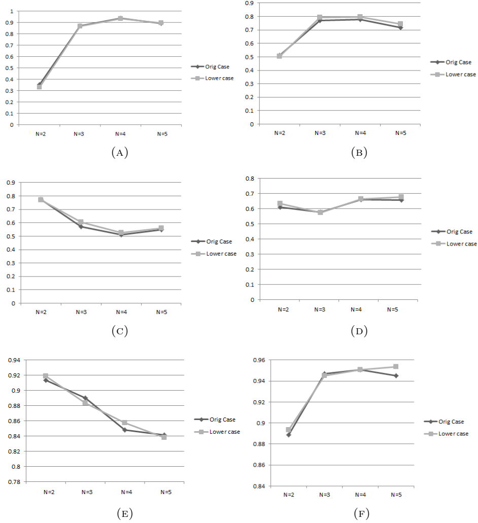
FIGURE 2. Variation of MAcc across different N-gram sizes ( N = 2 to 5 ) for all six classification methods: (A) SVM, (B) LR, (C) k-NN, (D) DT, (E) RF, and (F) ANN. This analysis examines how varying the N-gram size affects the models' performance. Values shown represent the average of the macro-accuracy scores computed over multiple experimental runs.
