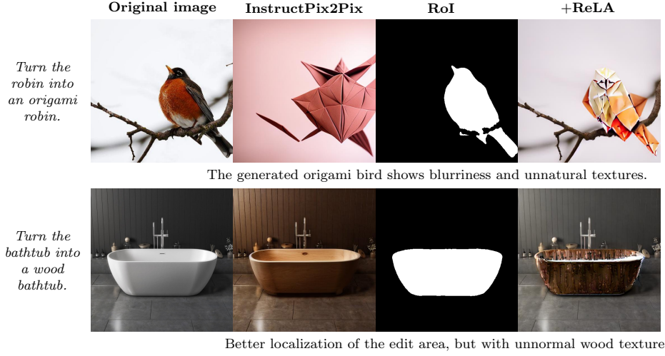
FIGURE 5. Examples of the images edited after integrating ReLA’s segmentation mask for cross-attention map regularization.
