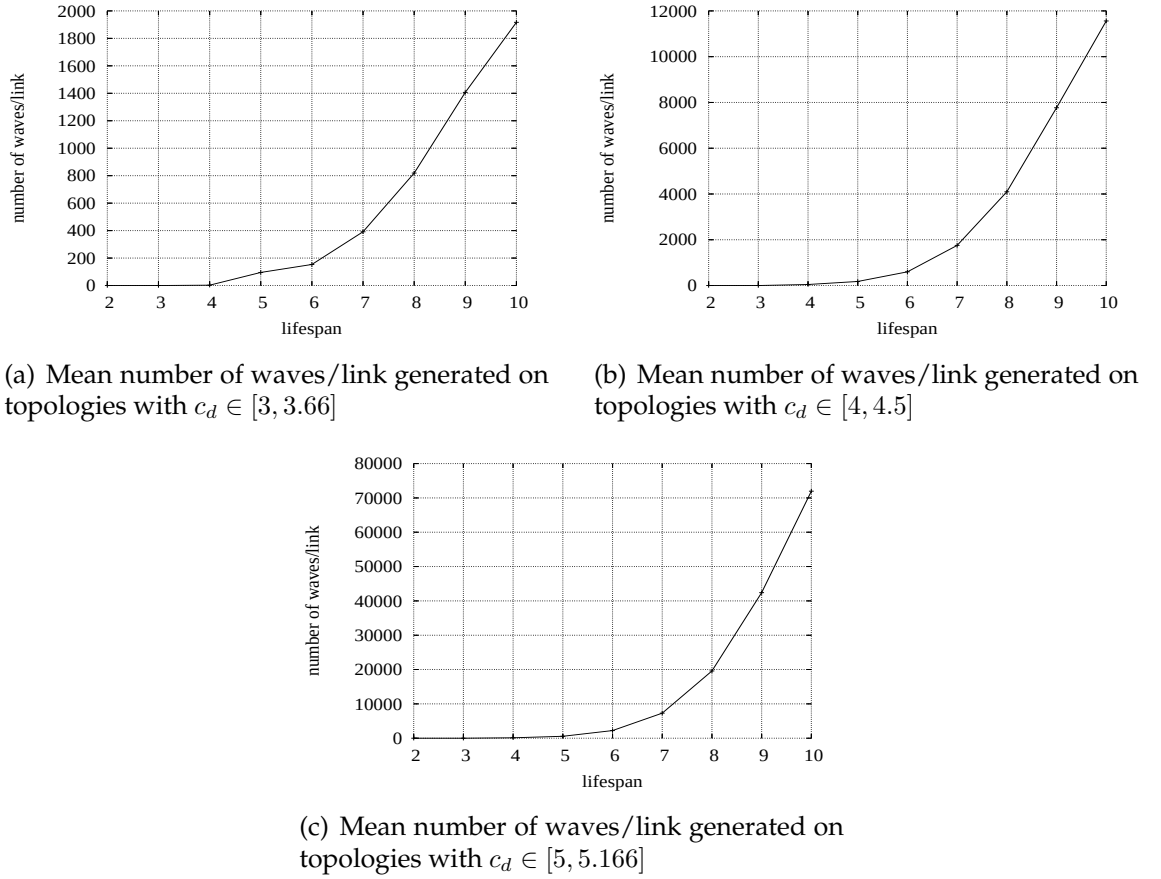
Figure 5.14: Macro-routing's communications overhead on different topologies
