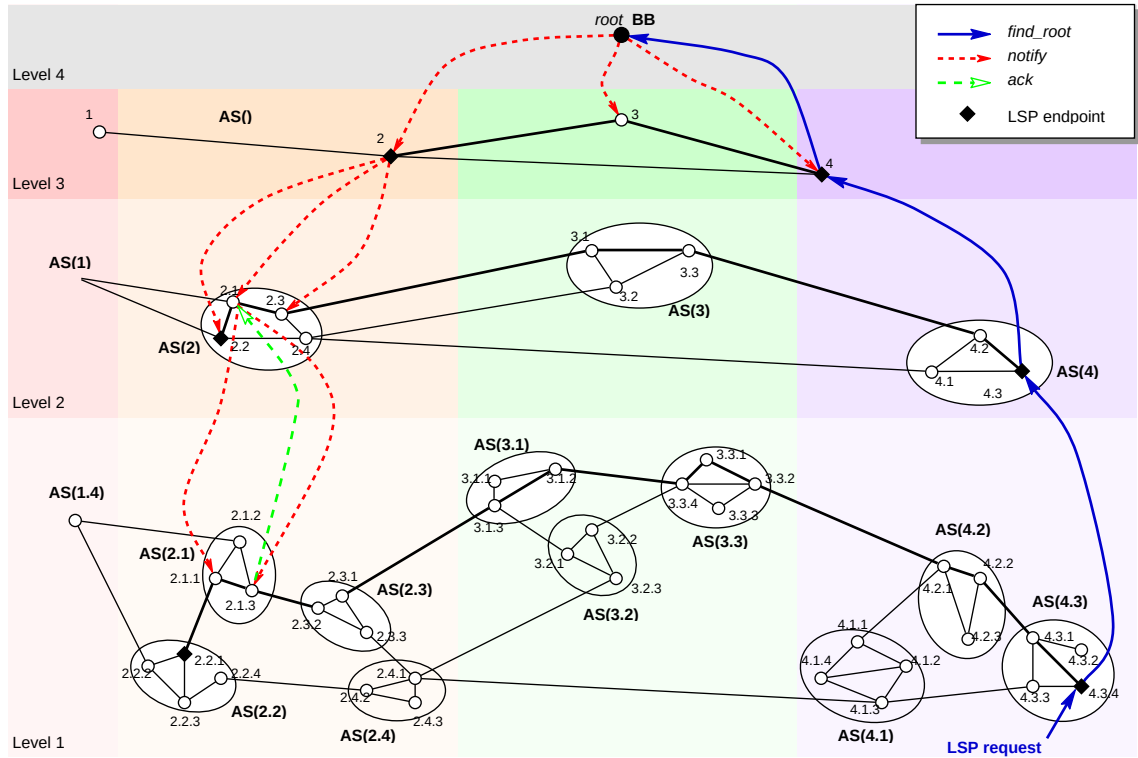
Figure 3.3: Hierarchical Distributed Protocol (HDP)
