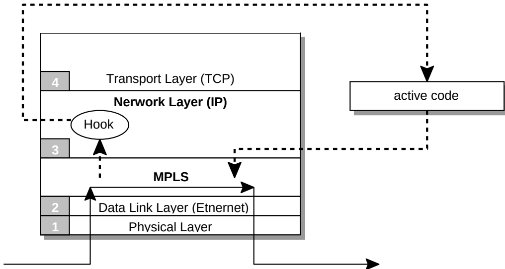
Figure 4.3: An active MPLS architecture
