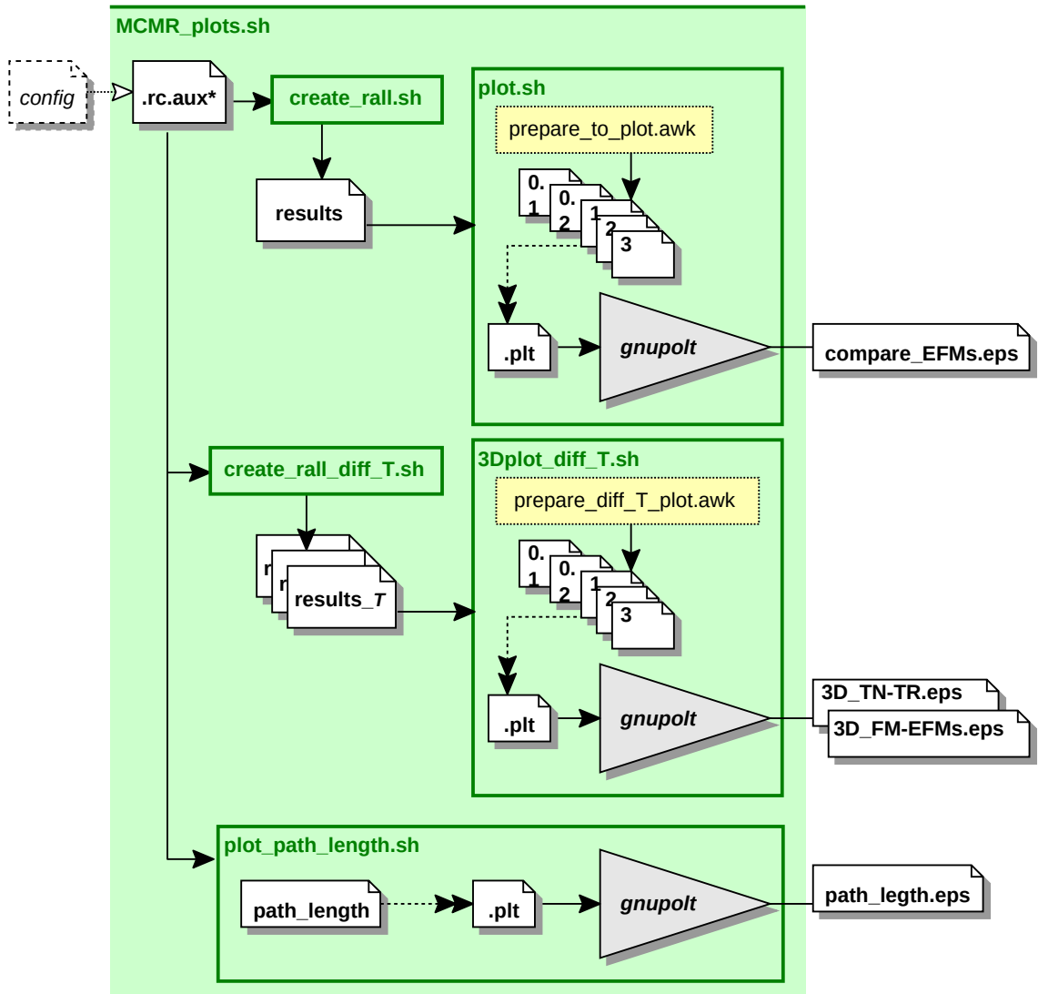
Figure E.11: The interpretation process for Multi-constraint Macro-routing's test results
