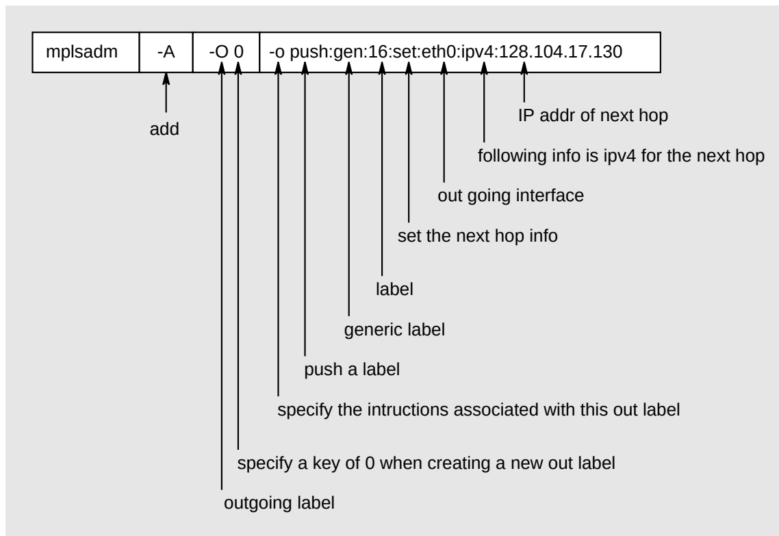
Figure B.2: Allocate / Establish an out-going label using mplsadm
