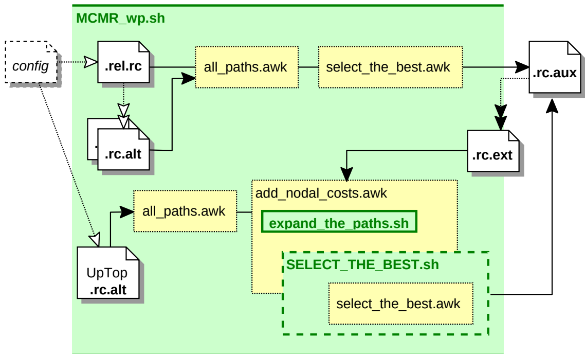
Figure E.8: The Multi-constrained Macro-routing model
