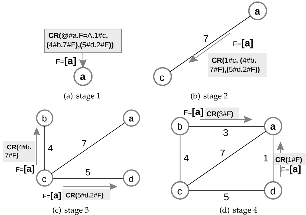
Figure A.4: Parallel creation of a four-nodes network topology
