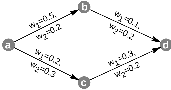
Figure 3.4: Counter-example for Jaffe's approximation algorithm
