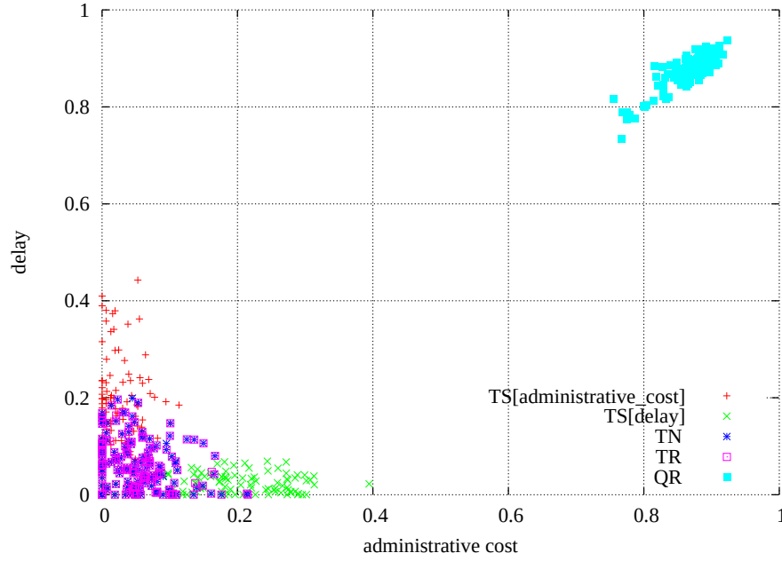
Figure 6.5: Comparing four of the EFM methods on a 20 \times 20 node topology
