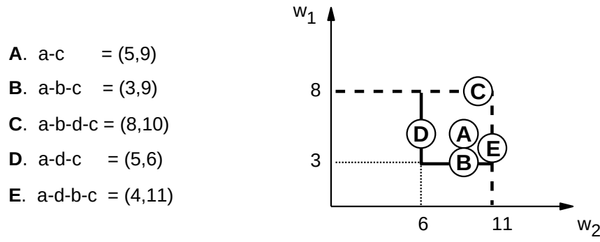
Figure 3.7: The representation of the paths into the QoS-metric bi-dimensional space
