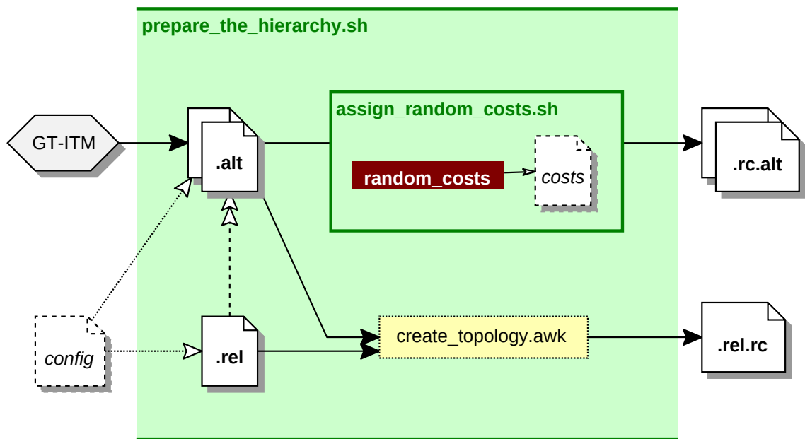
Figure E.4: Preparing the hierarchy diagram
