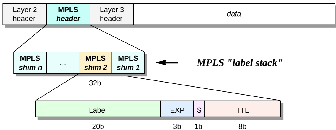
Figure 2.11: MPLS Label Stack
