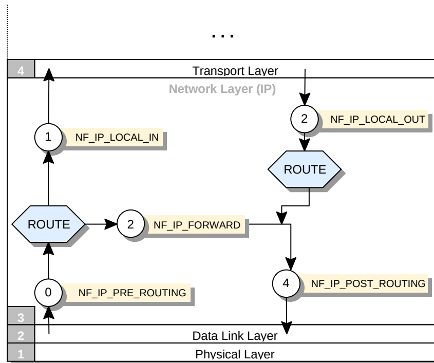
Figure C.1: The Netfilter hooks defined in IPv4
