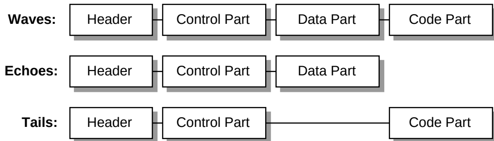
Figure A.7: The Wave Interpreter
