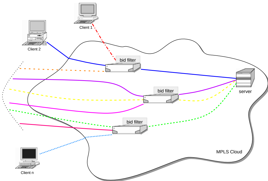
Figure 4.9: Online auction using bid filters
