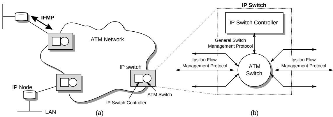
Figure 2.6: (a) An IP Switching Network (b) The structure of an IP Switch
