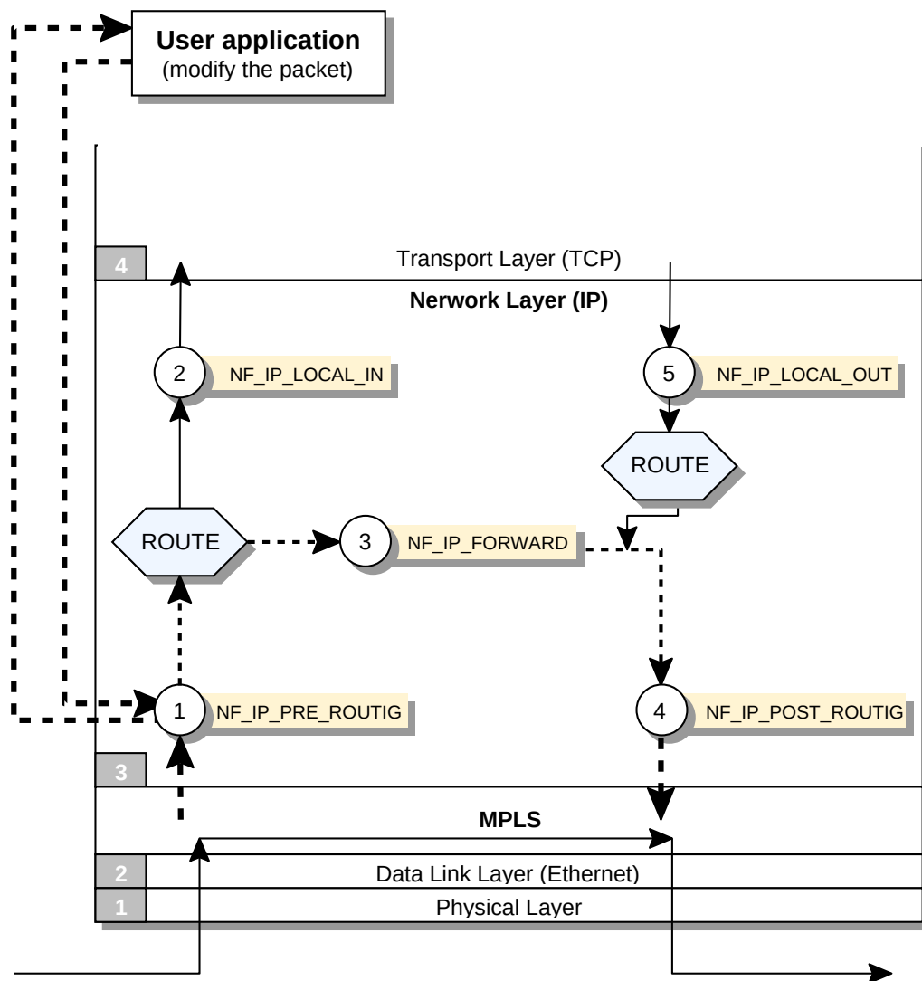
Figure 4.5: An MPLS node modified to programme the packets
