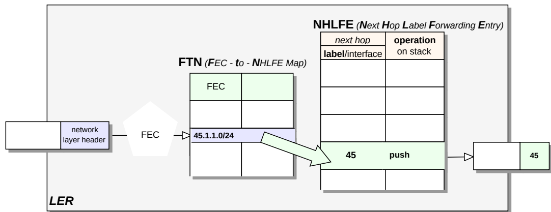
Figure 2.12: MPLS Data structures needed for an unlabelled packet
