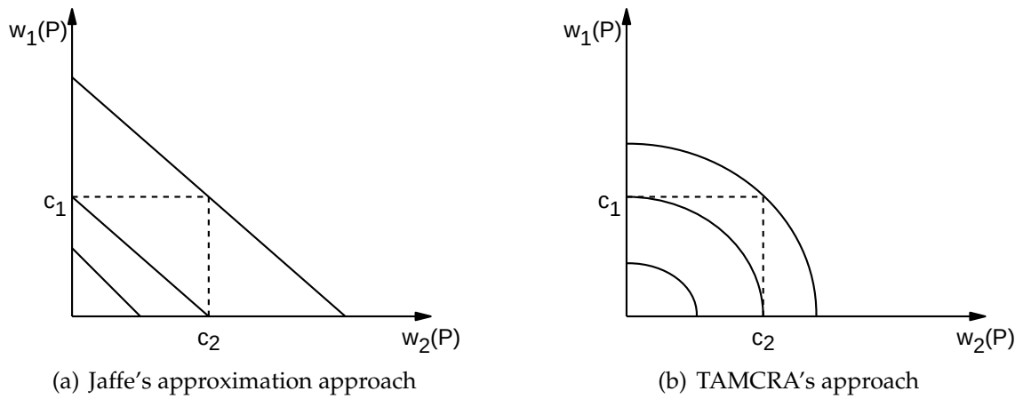
Figure 3.5: Searching a feasible path by minimising a linear composite function or a nonlinear composite function [98]
