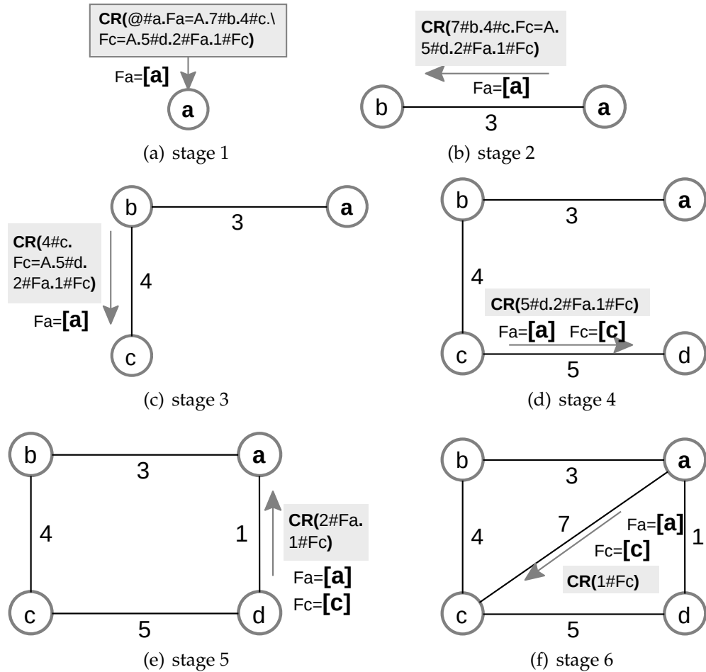
Figure A.3: Sequential creation of a four-nodes network topology
