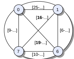
(e) the extended Full-Mesh
