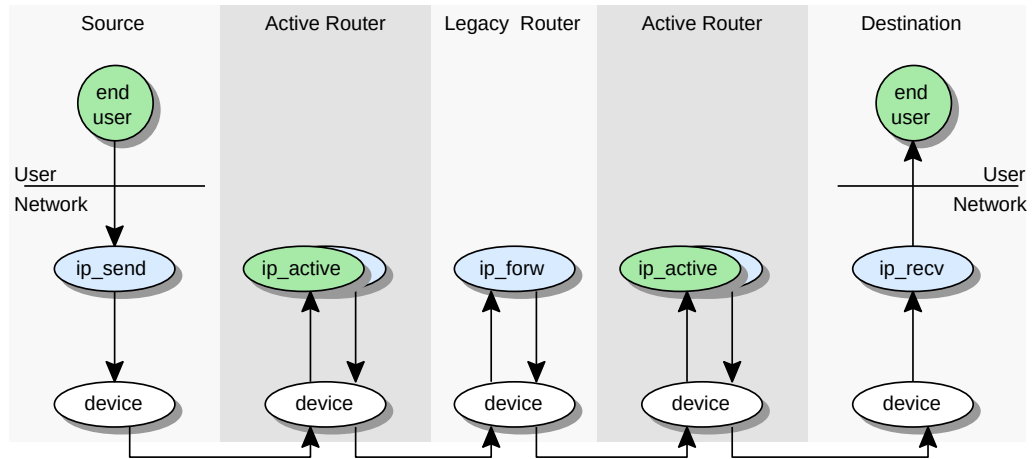
Figure 4.1: Packet processing within the nodes of a legacy Active Network
