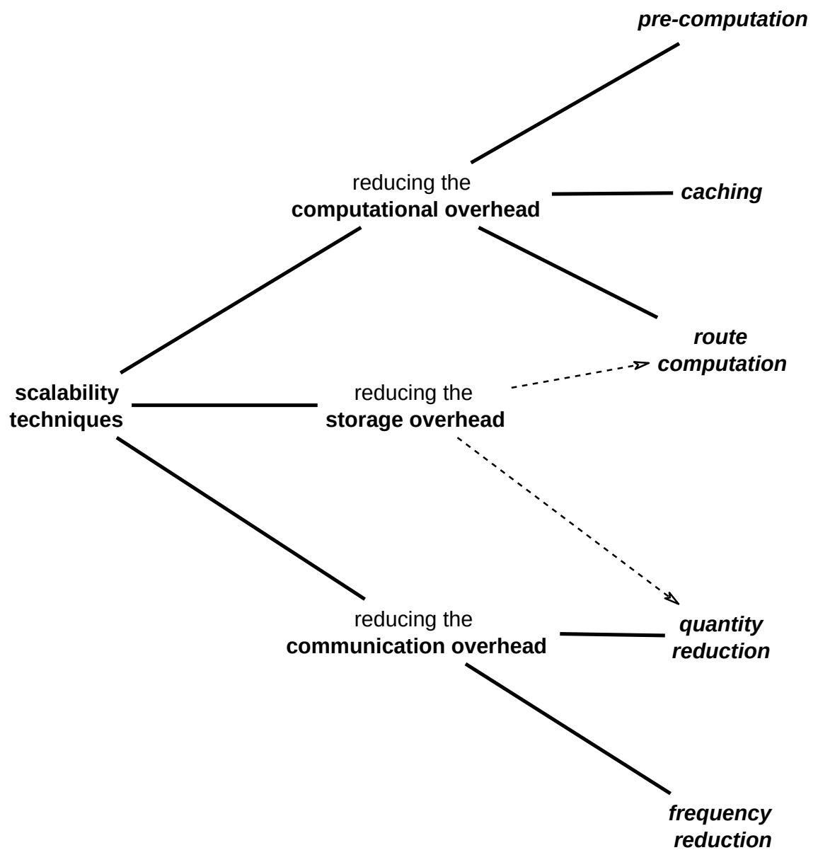
Figure 3.1: Techniques to enhance the QoS routing scalability
