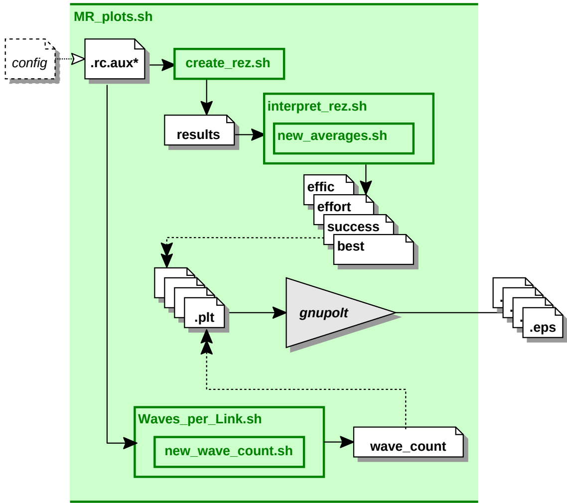
Figure E.9: The interpretation process for Macro-routing's test results
