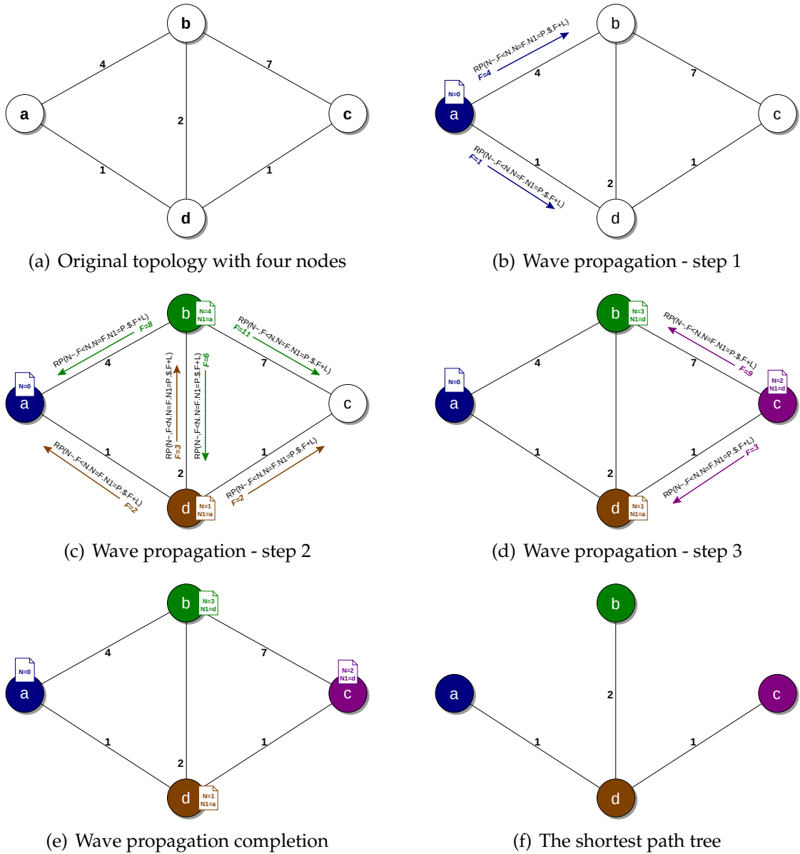
Figure 3.8: Using waves to find the shortest path tree
