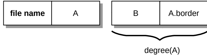
Figure E.7: Entry in the hierarchy specification file
