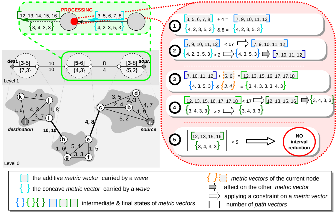
Figure 6.3: Example for two metrics (additive and concave)
