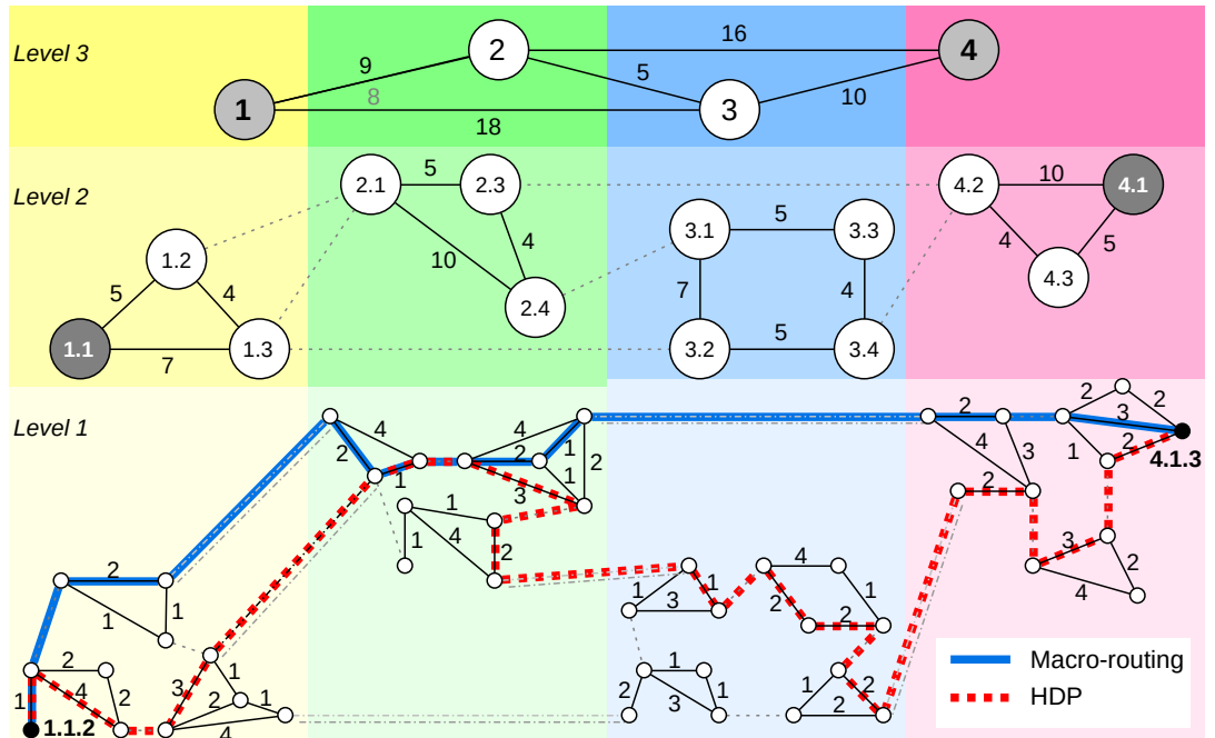
Figure 5.4: Macro-routing versus Hierarchical Distribution Protocol
