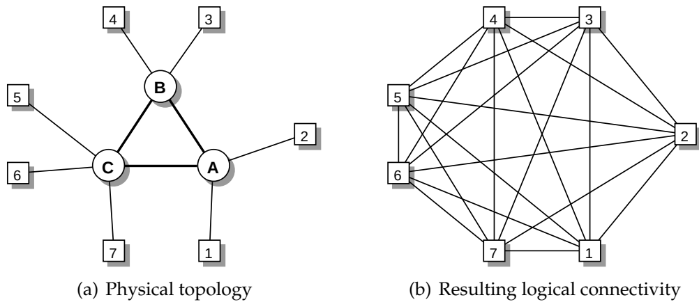
Figure 2.5: IP over ATM logical connectivity
