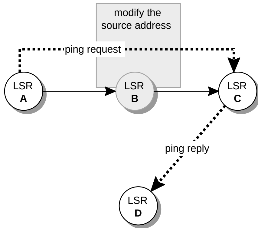
Figure 4.6: Our experiment test
