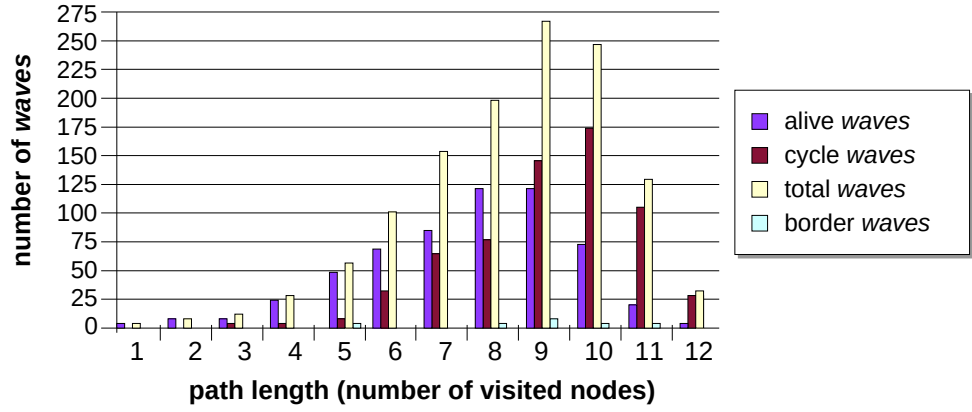
Figure 5.10: The number of waves propagating from a border node.
