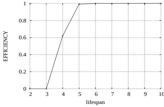
(a) Macro-routing's Mean Efficiency
