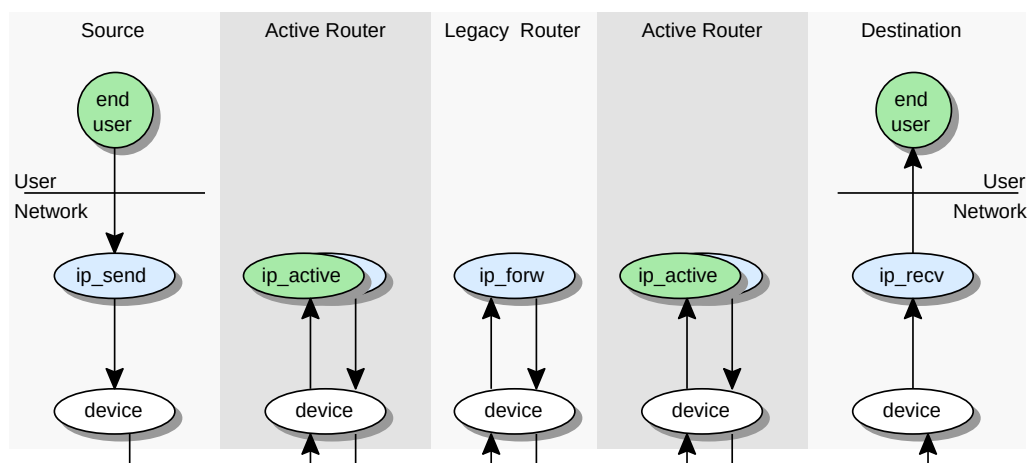
Figure 2.14: Application-specific processing within the nodes of an Active Network
