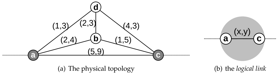
Figure 3.6: Example of topology aggregation considering two additive QoS metrics
