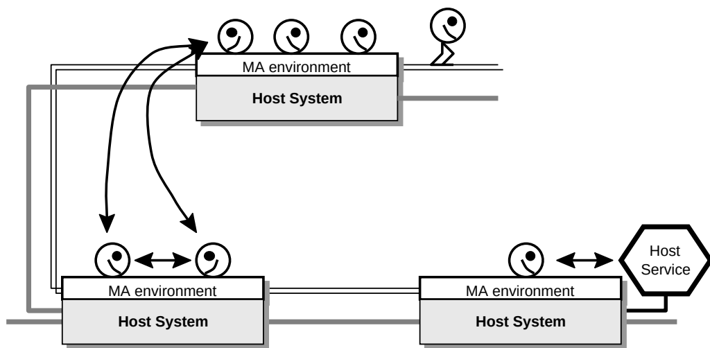
Figure 2.15: Basic mobile agent architecture
