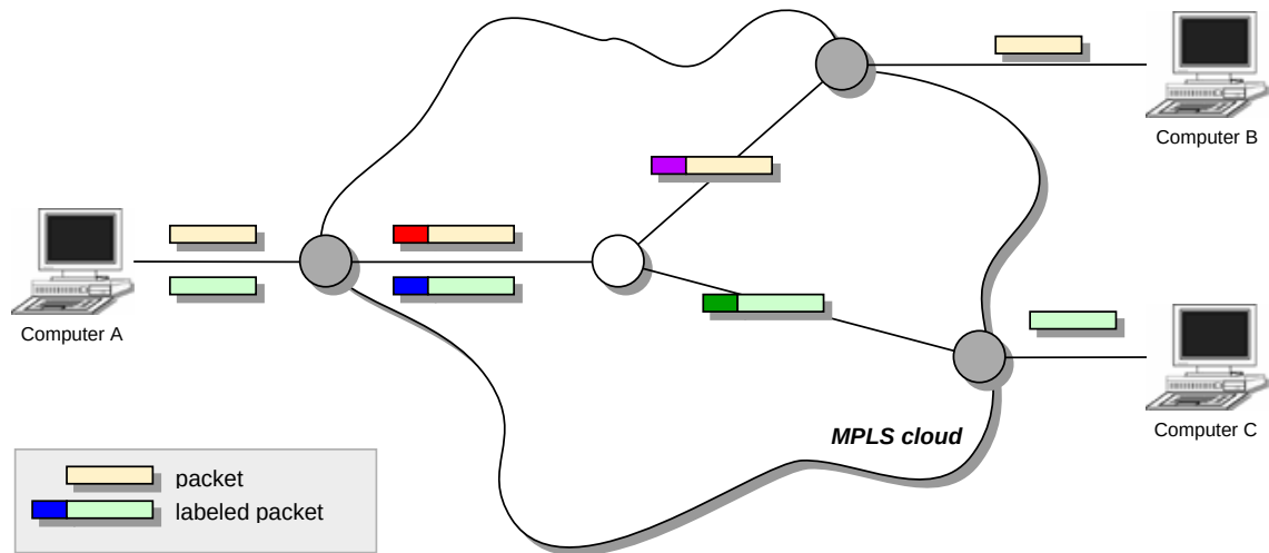
Figure 2.9: MPLS: Basic principles
