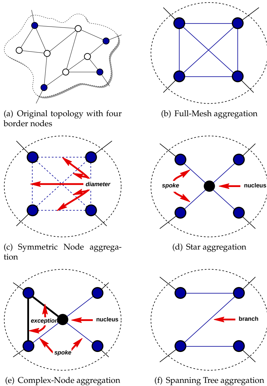
Figure 3.2: Examples of topology aggregation methods
