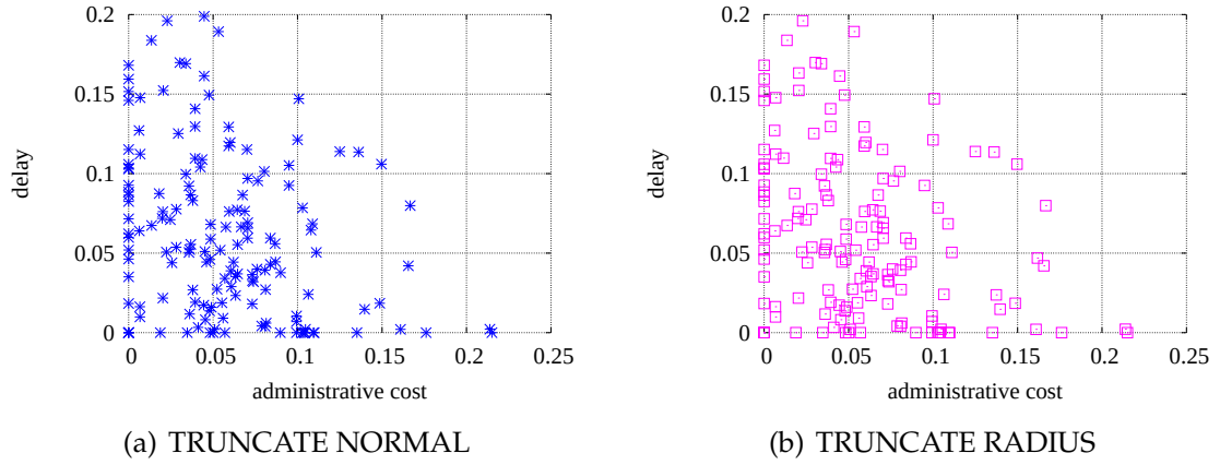
Figure 6.8: Detailed comparison of TN and TR methods on a 20 \times 20 node topology
