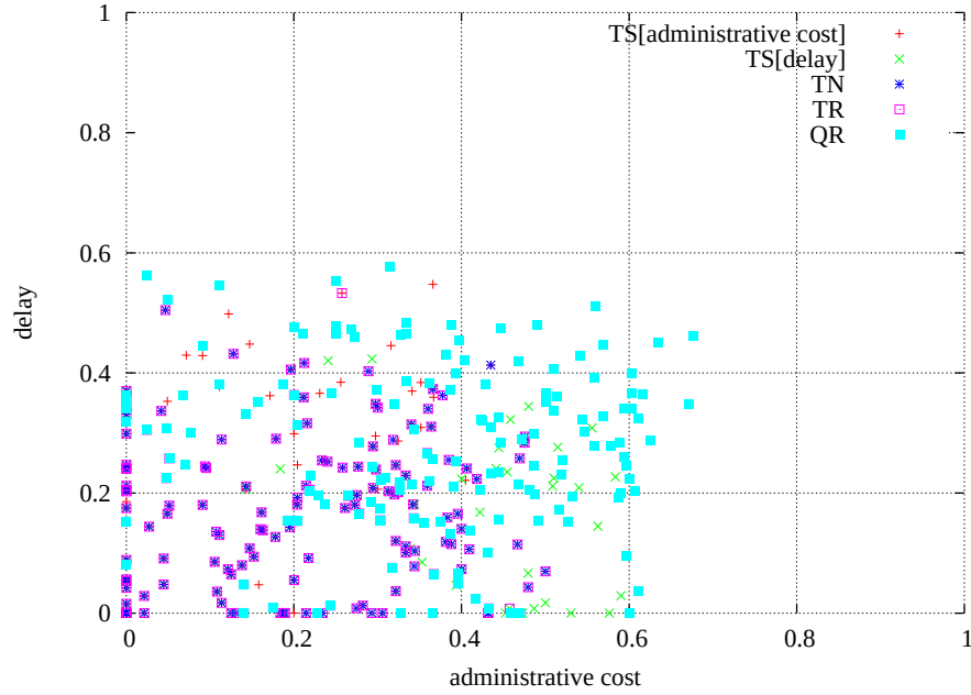
Figure 6.7: A comparison of four of the EFM methods on a 4 \times 4 node topology
