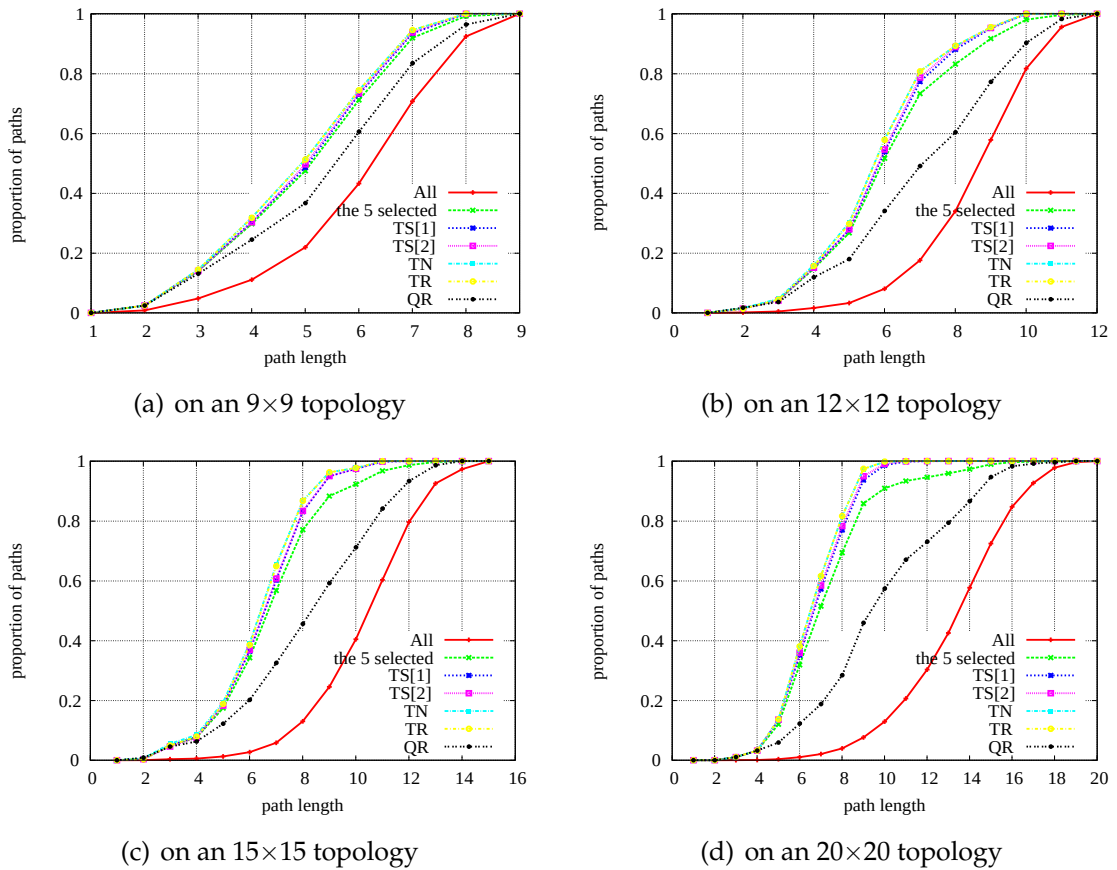
Figure 6.11: The convergence of all and the 5th selected paths in terms of lifespan
