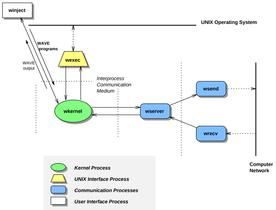
Figure A.5: The Wave Interpreter
