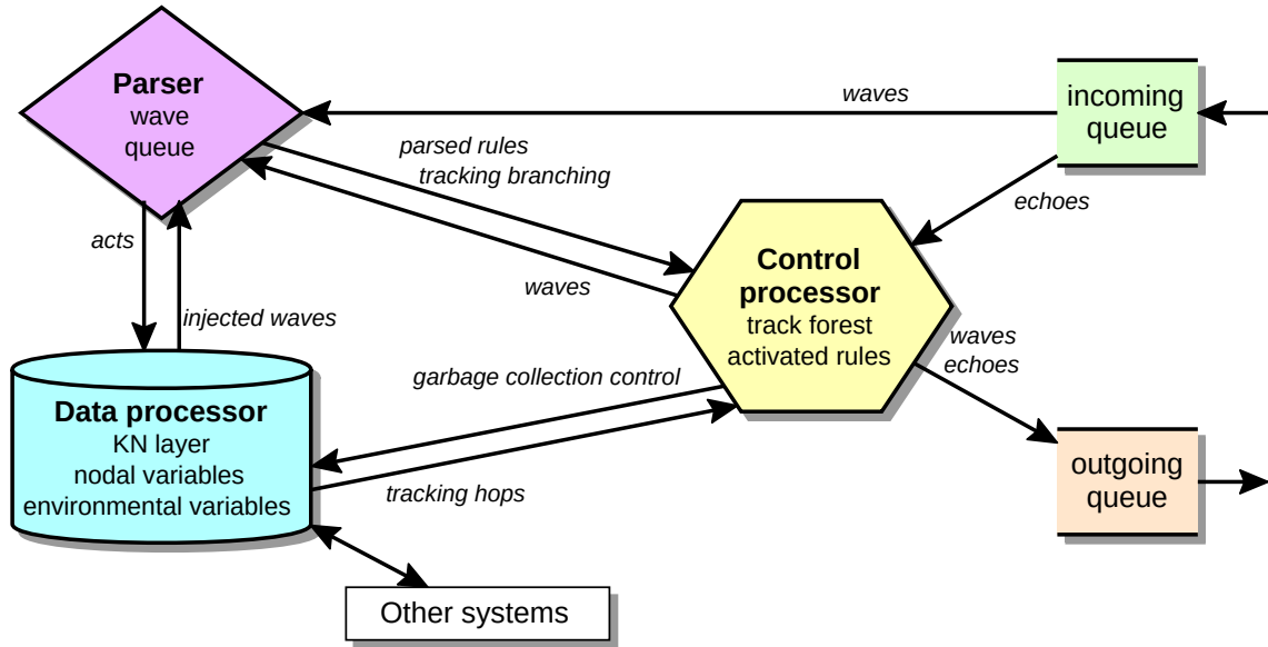
Figure A.6: The Wave Interpreter Architecture
