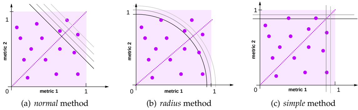
Figure 6.4: Methods for truncating a two-dimensional EFM interval
