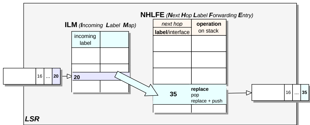
Figure 2.13: MPLS Data structures needed for an labelled packet
