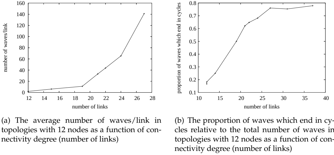
Figure 5.9: The wave population evolution on different topologies as a function of connectivity (i.e. number of links)
