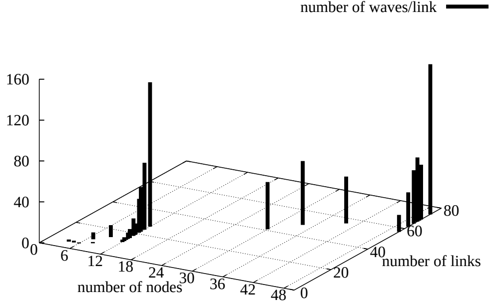
Figure 5.8: Number of waves/link in various topologies
