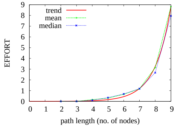
(a) N = 9 and L = \overline{8, 36}
