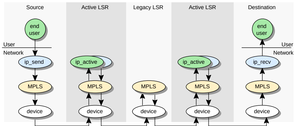
Figure 4.2: Packet processing within the nodes of an MPLS Active Network
