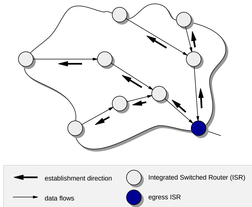
Figure 2.7: IBM ARIS Switched Paths
