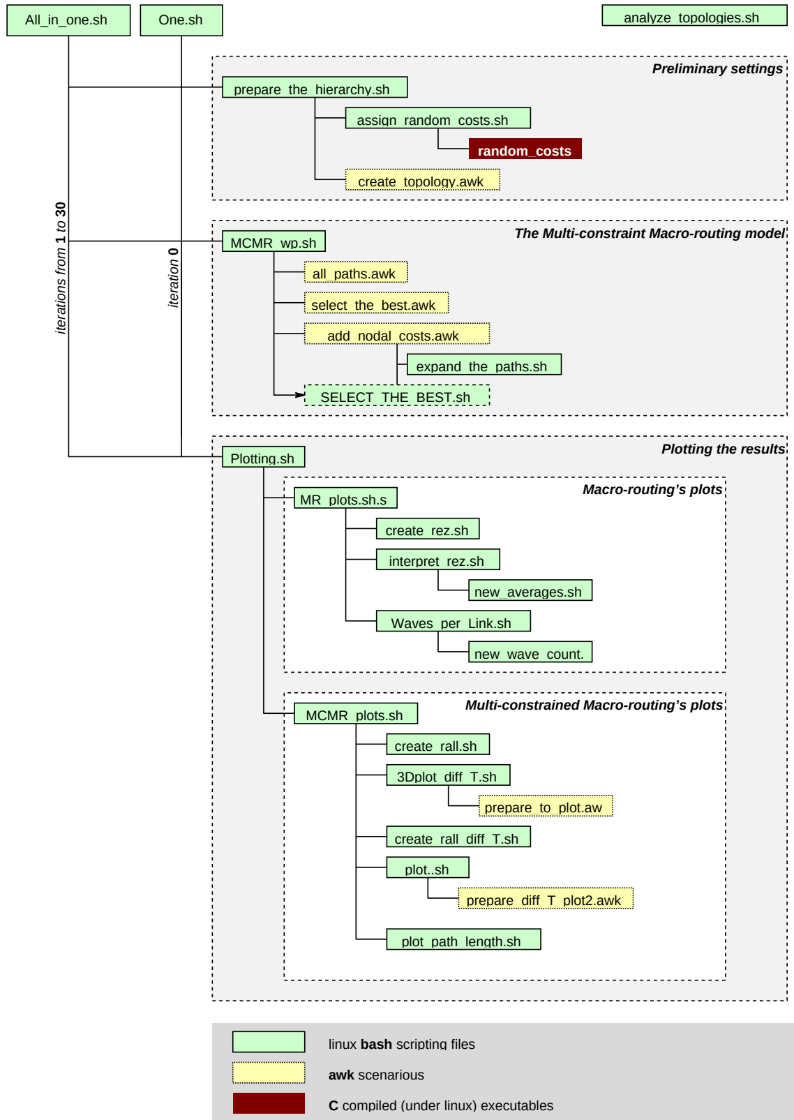
Figure E.1: The Linux application generating the Multi-constrained Macro-routing paths
