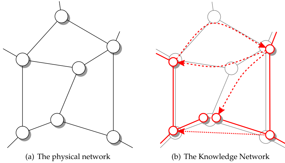
Figure A.1: The mapping of the Knowledge Network on the physical network
