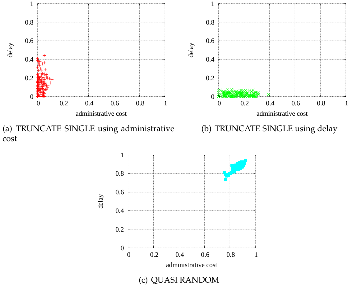
Figure 6.6: Detailed comparison of TS[administrativecost] , TS[delay] and QR methods on a 20 \times 20 node topology
