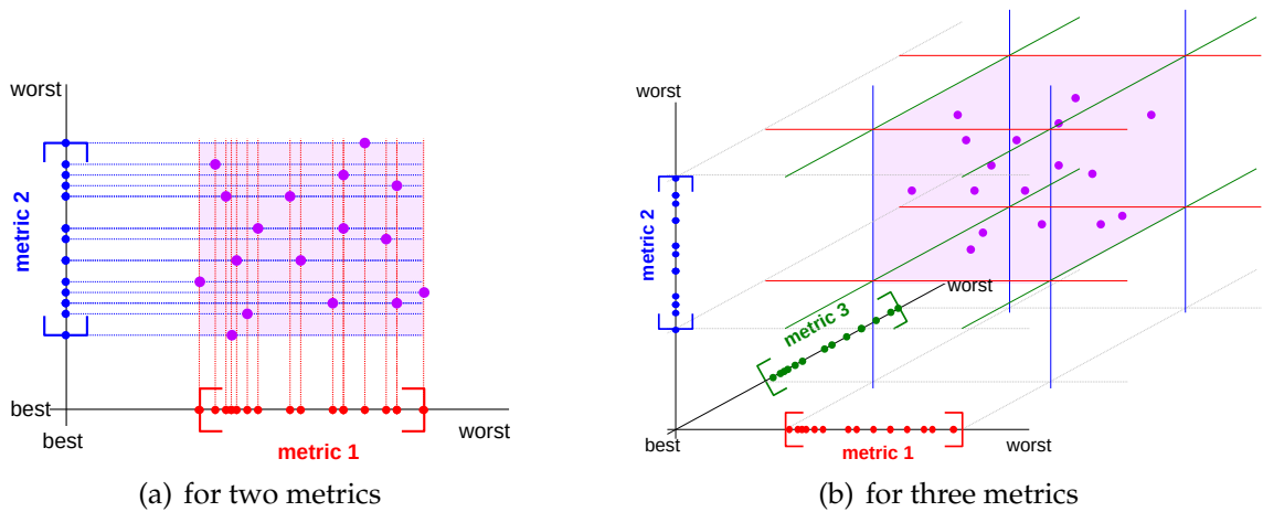
Figure 6.2: Visualization of the cost matrix
