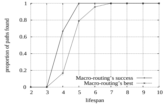
(b) Mean proportion of success and best Macro-routing paths found
