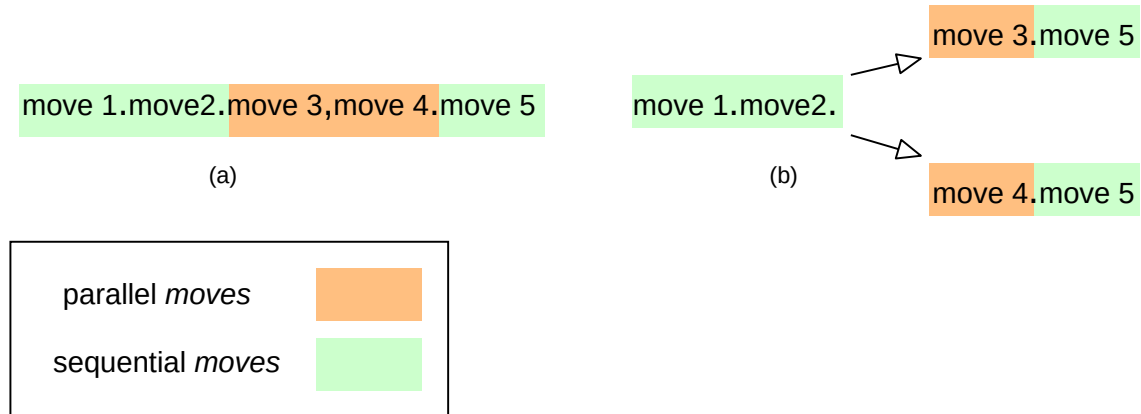
Figure 2.17: (a) a Wave structure (b) seen by the Wave interpreter
