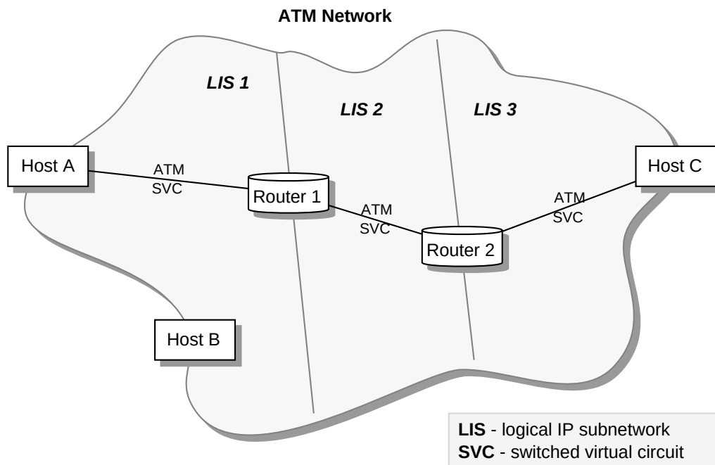
Figure 2.4: Multiple IP LIS's on one ATM network
