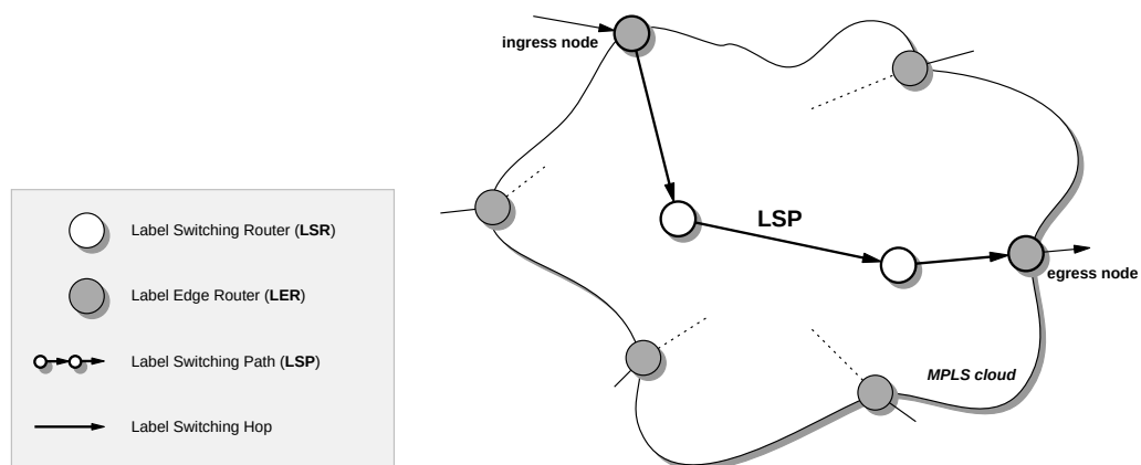
Figure 2.8: The MPLS cloud and its main components
