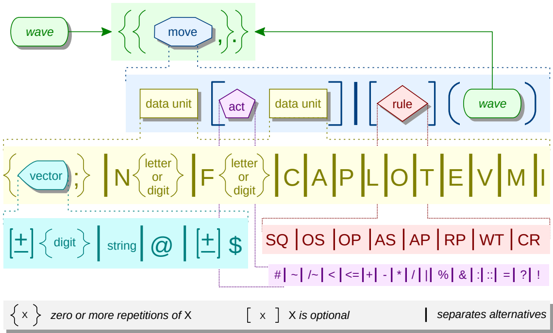
Figure A.2: The syntax of the Wave Language
