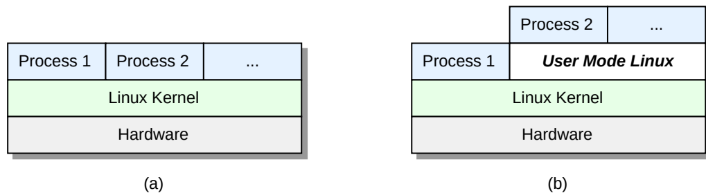
Figure B.3: (a) The Linux Kernel (b) The User-Mode Linux Kernel
