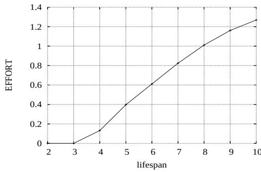
(c) Macro-routing's Mean Effort
