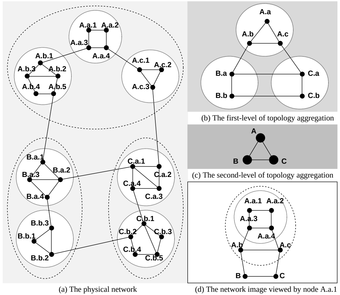
Figure 2.3: A hierarchical network model
