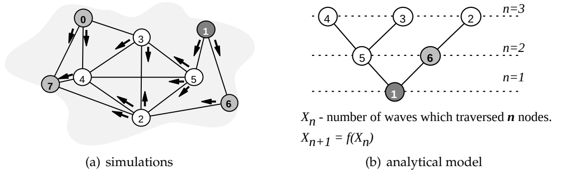
Figure 5.5: Wave counting tests
