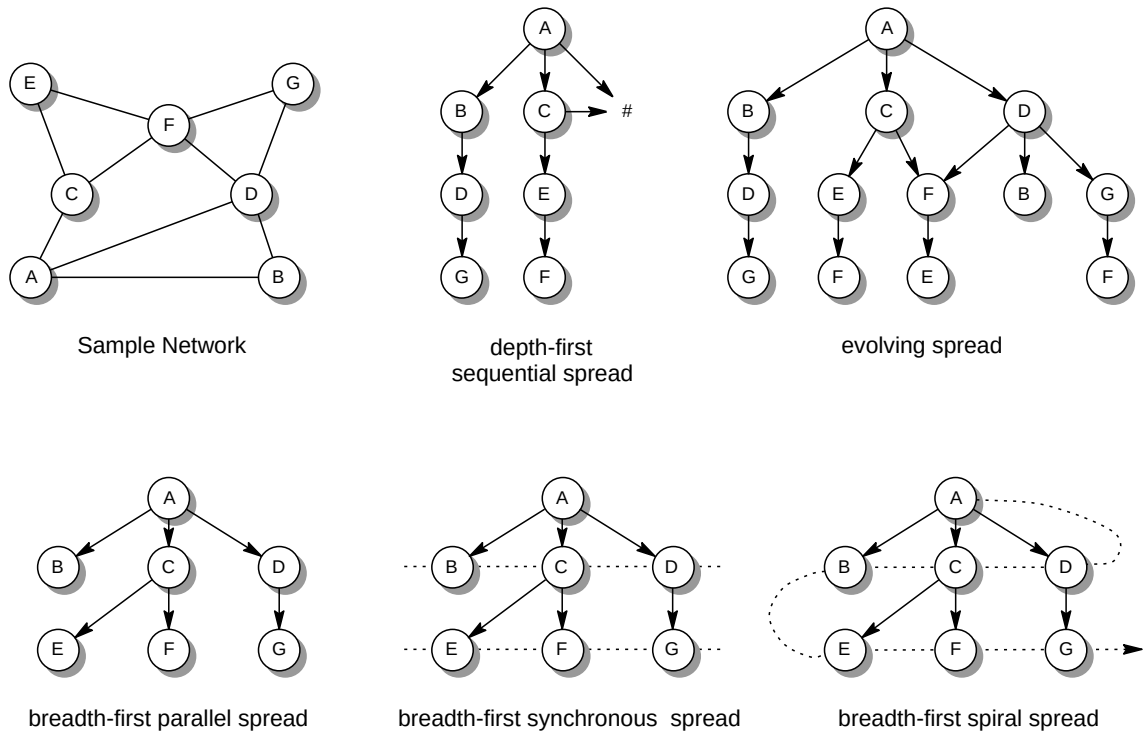
Figure 2.18: Basic Space Navigation Mechanisms in Wave
