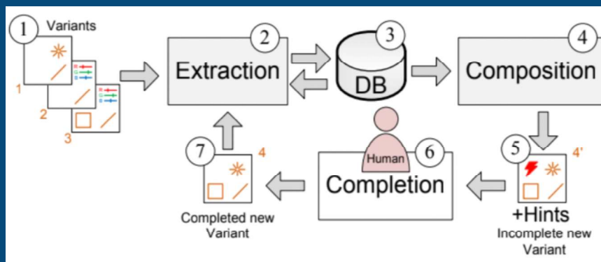
Extraction and Composition for Clone-and-Own (ECCO) Workflow
