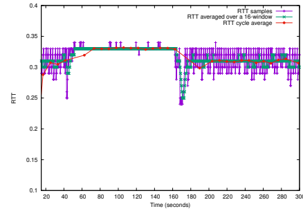
Fig. 2. The two-stages smoothing performed on RTT samples
