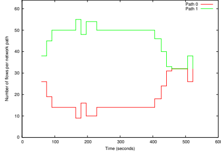
Fig. 4. The number of multihoming flows mapped on each path by the multihoming routing algorithm; DropTail queuing and 100Mbps capacity
