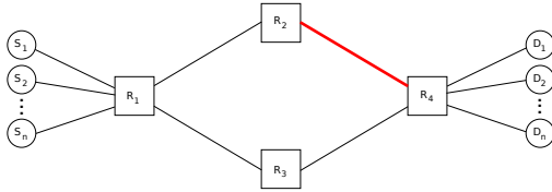
Fig. 3. The network setup used in the experiments
