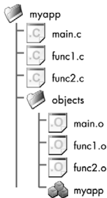
Figure 1: Putting built object files in a subdirectory
